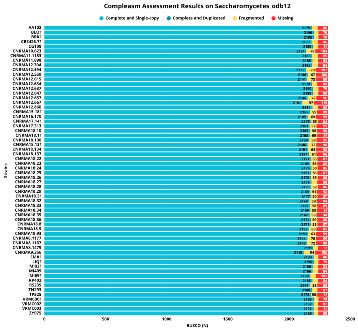
Fig. S1. Compleasm results on Saccharomyces_odb12 database of the genome assemblies included in the pangenome graph.
