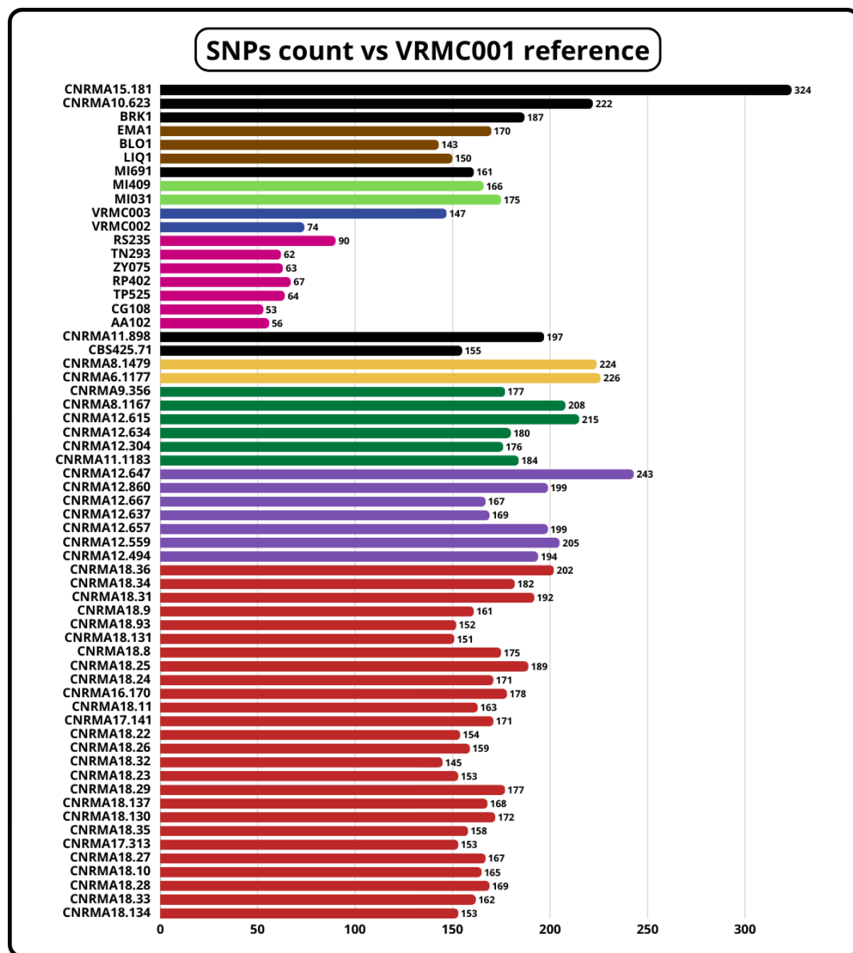
Fig. S2. Number of SNPs in the investigated M. clavatus strains relative to the reference strain VRMC001.
